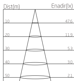
150W-Lux Distance Curve
