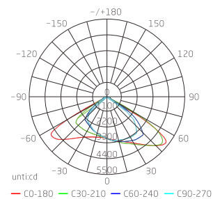
150W-Light Distribution Curve
